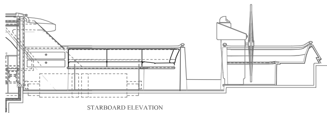
STARBOARD ELEVATION
